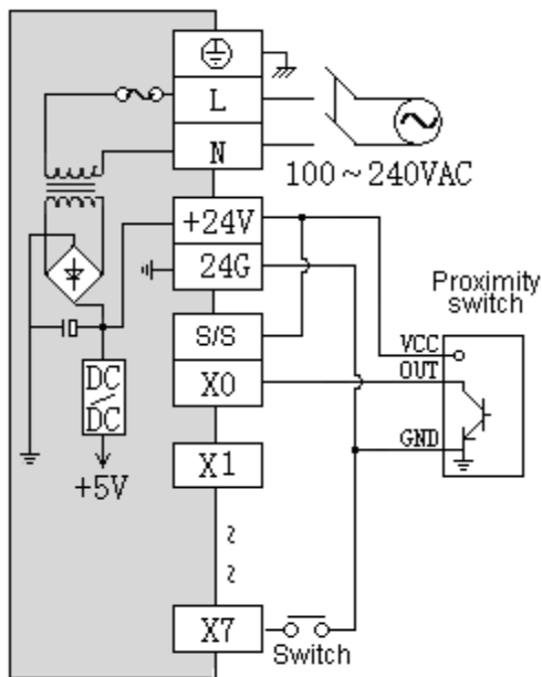
NPN Internal power
