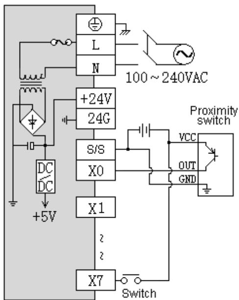
PNP External power
