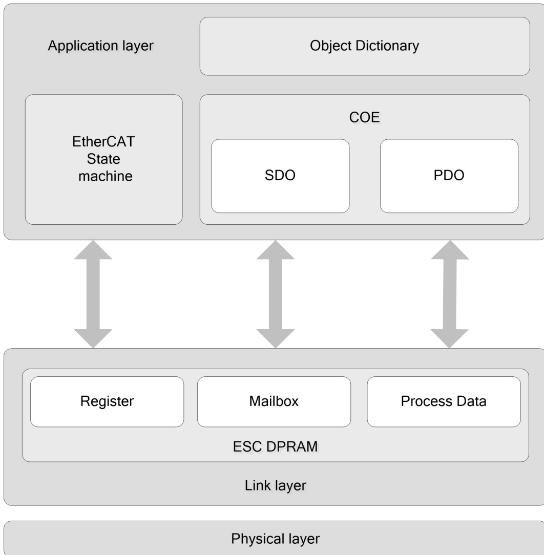
Figure3-1 Communication structure
