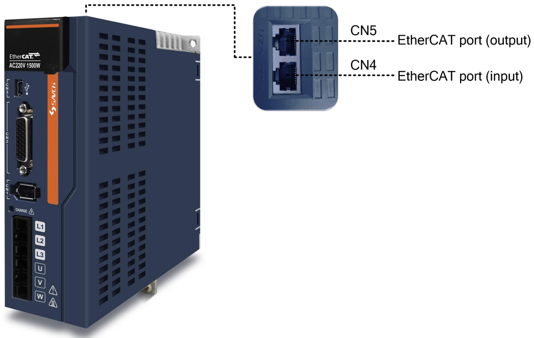
Figure 2-1 Names of EtherCAT port
